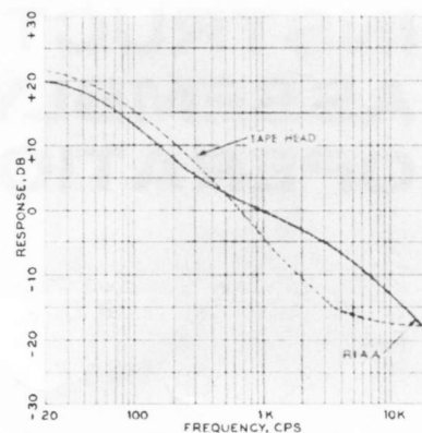
Equalization.
