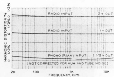
Harmonic distortion percentage.
