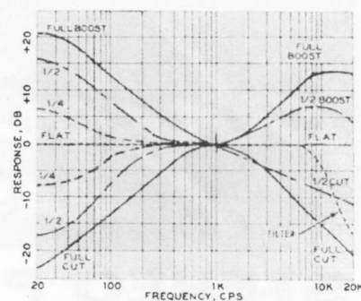
Contours of the tone controls.
